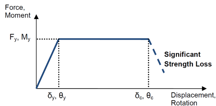
Fig. 3: Force/Moment versus displacement/rotation minimum backbone modelling requirements.
